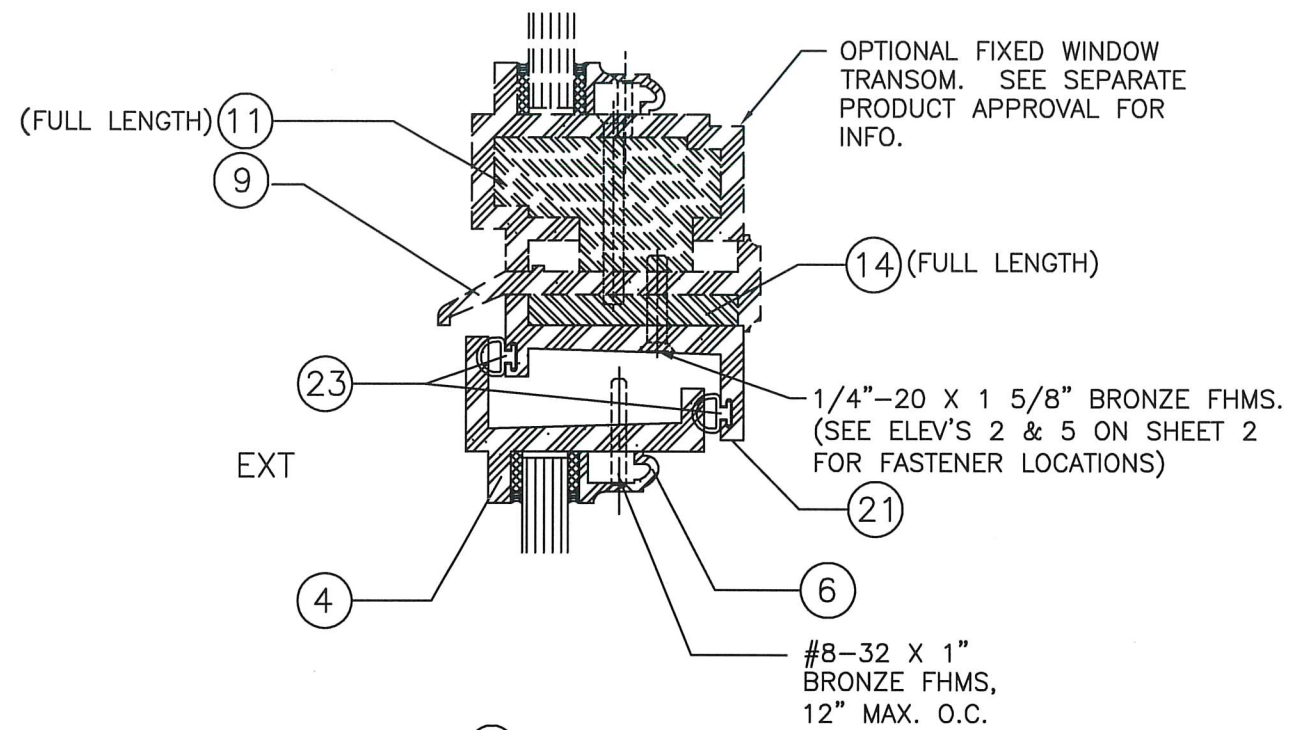
(B) TRANSOM (ELEV'S 2/2 OR 5/2)
