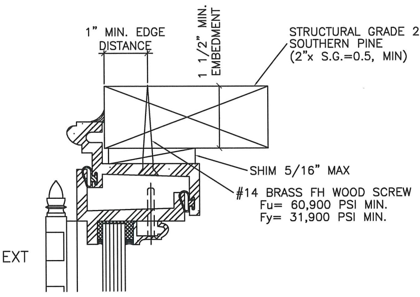
③ MOUNT TO WOOD
