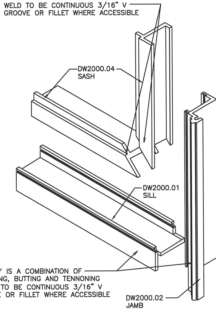
EXPLODED ISOMETRIC
