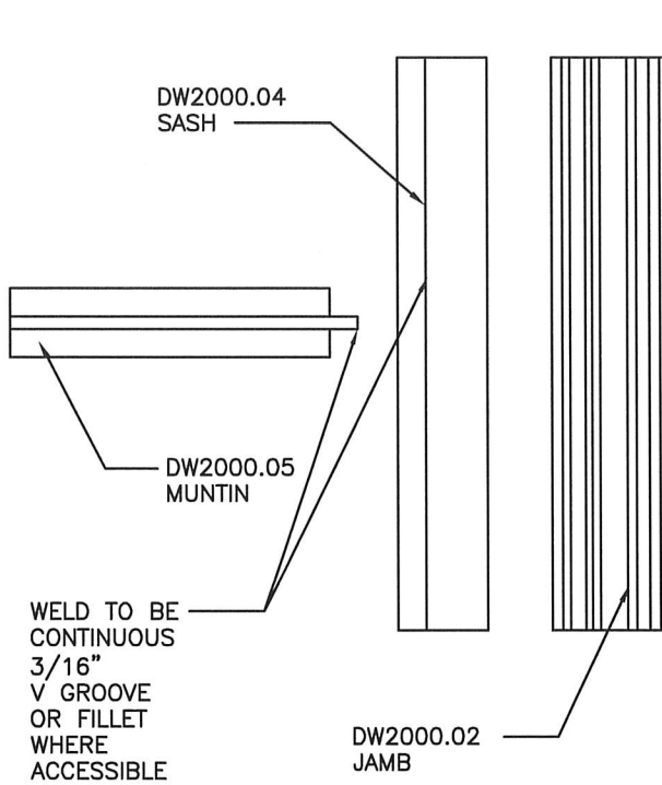
EXPLODED ELEVATION
