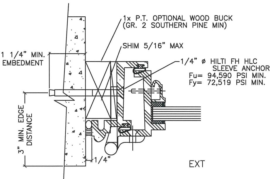
④ MOUNT TO CMU OPTIONAL WOOD BUCK (JAMB ONLY)
