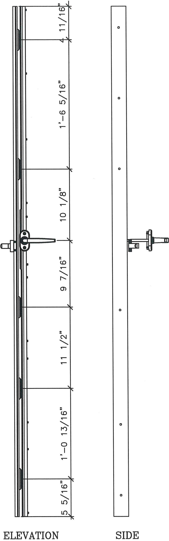
1 DW.2009.WLS-05 HACI MULTI-POINT LEVER LOCK
