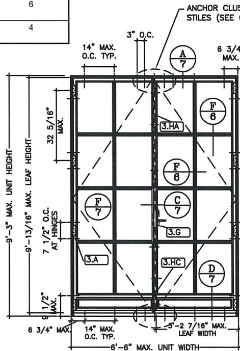
4 OUTSWING PAIR WITH OPTIONAL KICKPLATE LOCK OPTION 3 SHOWN (EXTERIOR VIEW)
