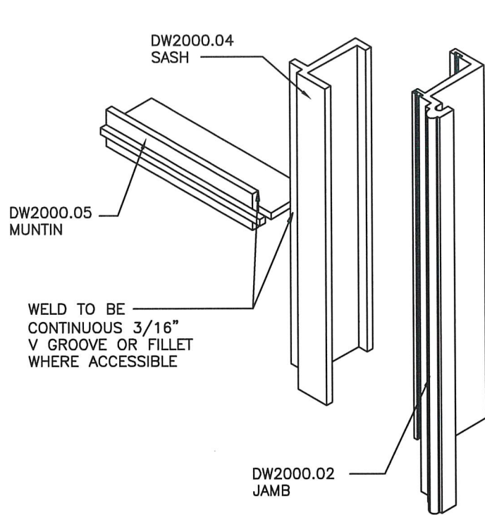
EXPLODED ISOMETRIC
