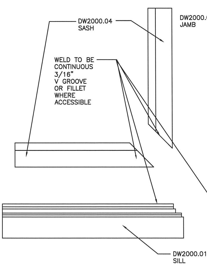
EXPLODED ELEVATION
