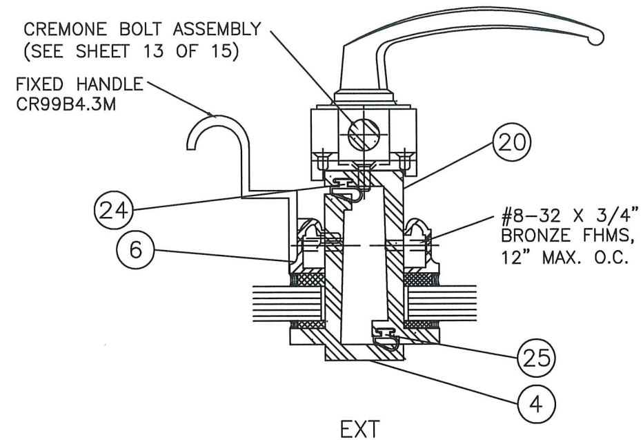
(C) MEETING STILE
