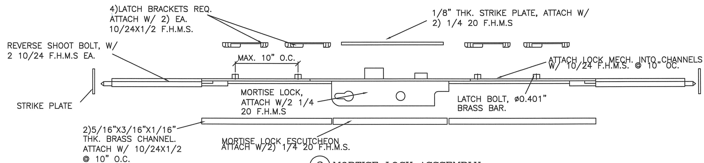
2 MORTISE LOCK ASSEMBLY
