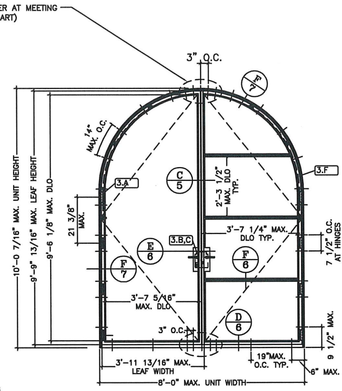
3 OUTSWING PAIR WITH ROUND TOP LOCK OPTION 6 SHOWN (EXTERIOR VIEW)
