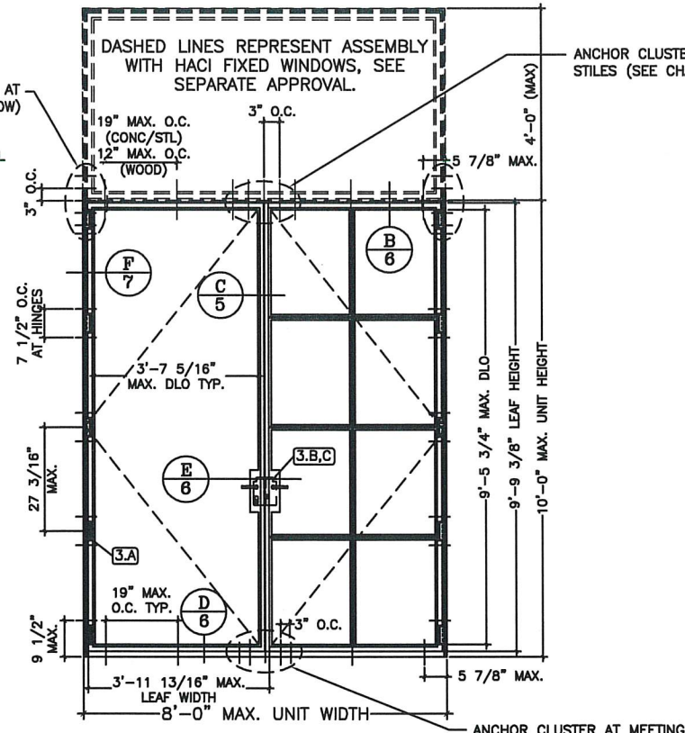
2 OUTSWING PAIR WITH TRANSOM LOCK OPTION 4 SHOWN (EXTERIOR VIEW)
