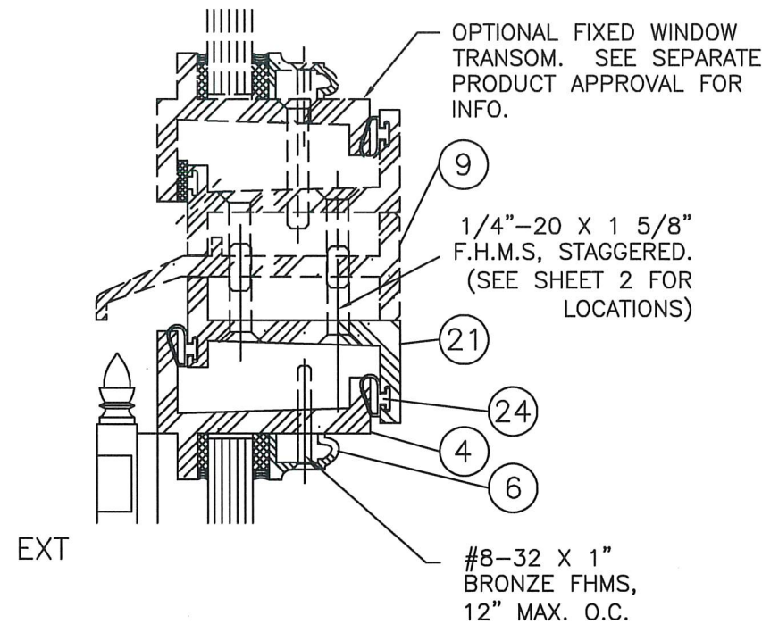
(B) HEAD/TRANSOM (ELEV. 5/2 ONLY)
