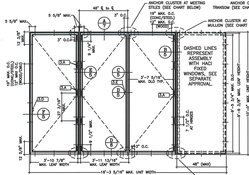
1 OUTSWING PAIR MULLED WITH SINGLE AND FIXED SIDELITE LOCK OPTIONS 5 (PAIR) AND 1 (SINGLE) SHOWN (EXTERIOR VIEW)
