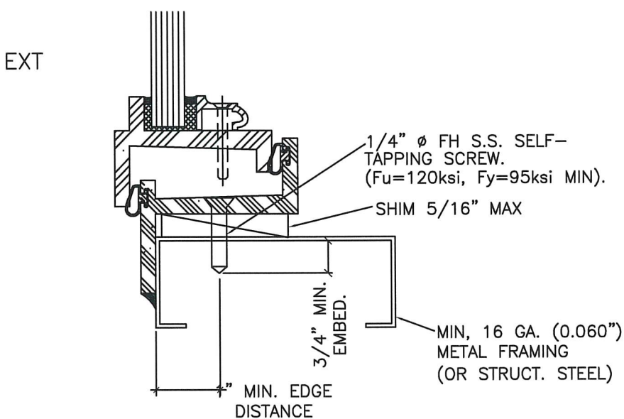
⑤ MOUNT TO METAL STUD
