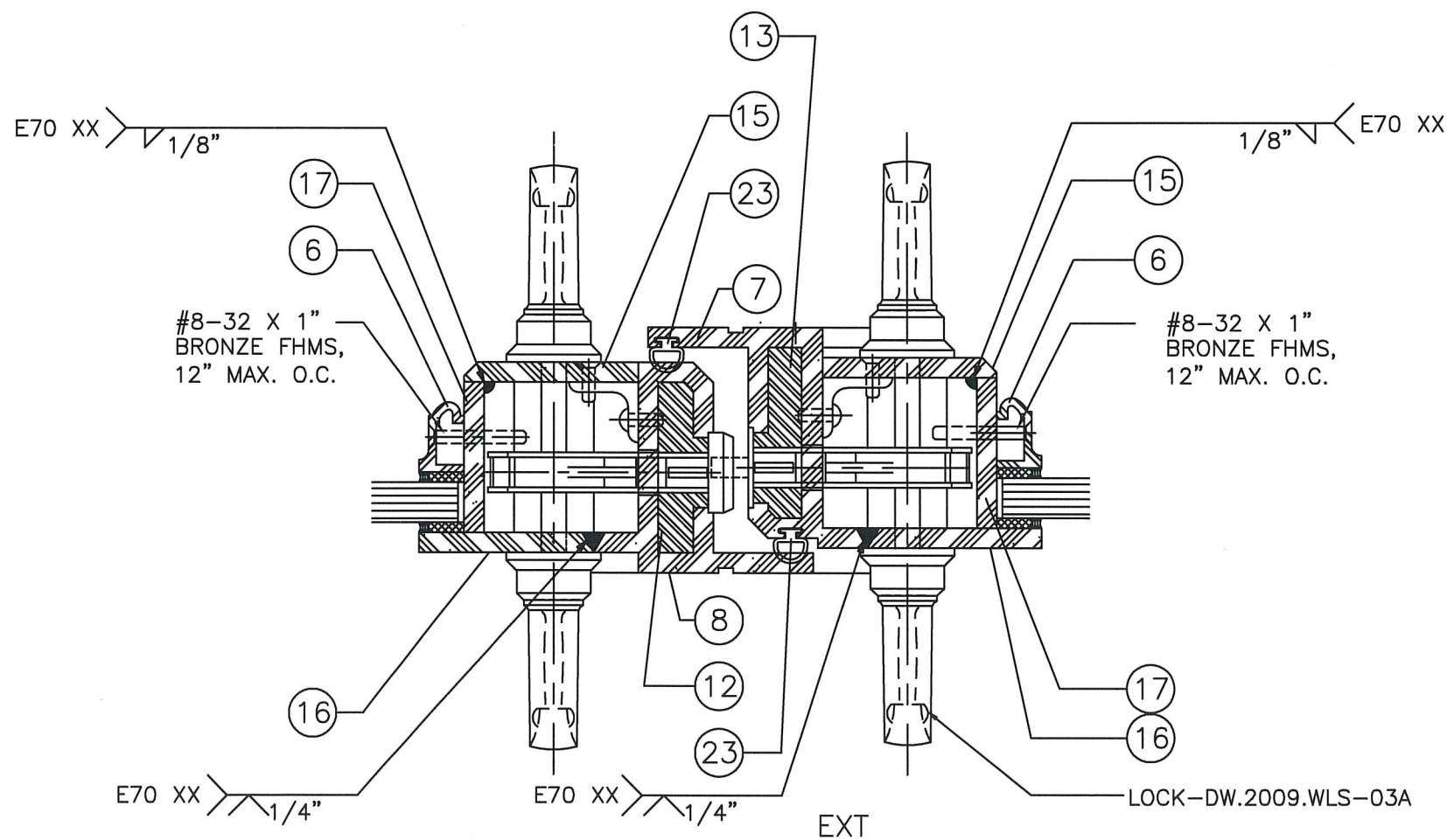
(E) MEETING STILE
