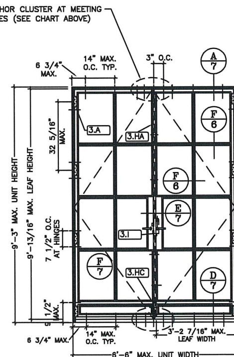
6 OUTSWING PAIR WITH OPTIONAL KICKPLATE LOCK OPTION 2 SHOWN (EXTERIOR VIEW)
