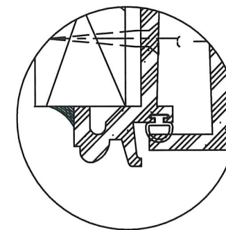
4 APPLIED BRICK MOLDING
