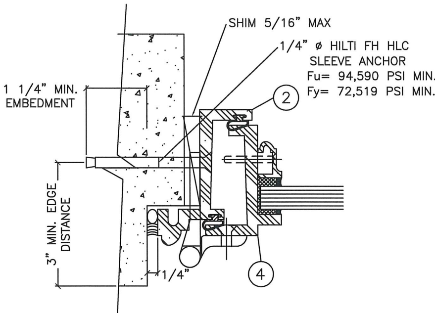
② MOUNT TO CONCRETE
