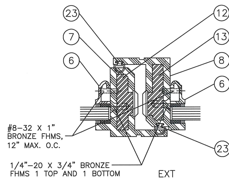
© MEETING STILE
