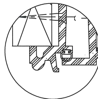
3 STANDARD BRICK MOLDING
