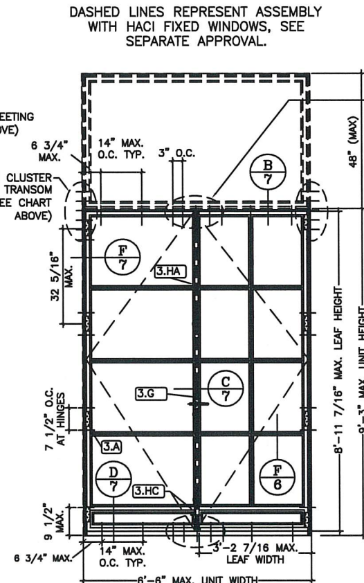
5 OUTSWING PAIR WITH TRANSOM AND OPTIONAL KICKPLATE LOCK OPTION 3 SHOWN (EXTERIOR VIEW)
