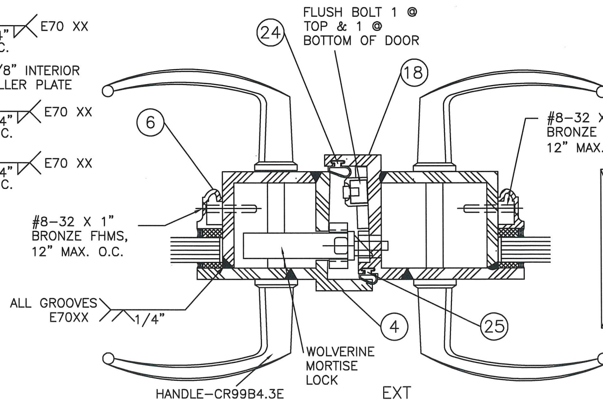
(E) MORTISE LOCK
